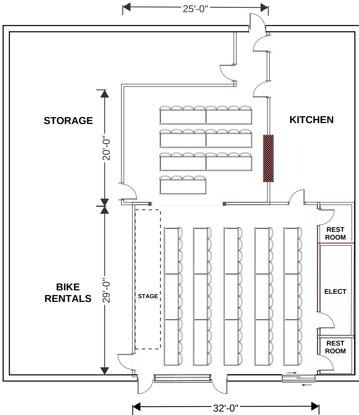
THE SAND SHACK 1428 SQUARE FEET ONE CLASSROOM CONFIGURATION SEATS UP TO 90 GUESTS PLUS 10 PRESENTERS
