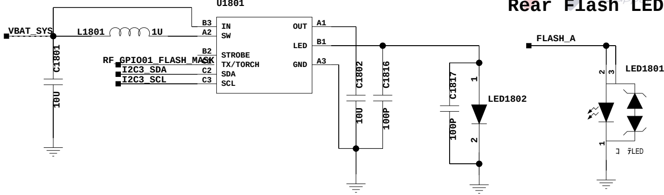
IR LED
