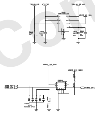
UIM2 Connector
