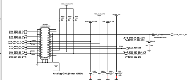
8M_CAM Connector (MIPI)
