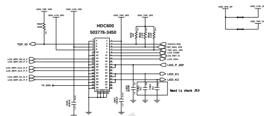
LCD Connector(5")
