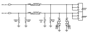
Speaker
