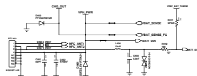
Battery Connector
