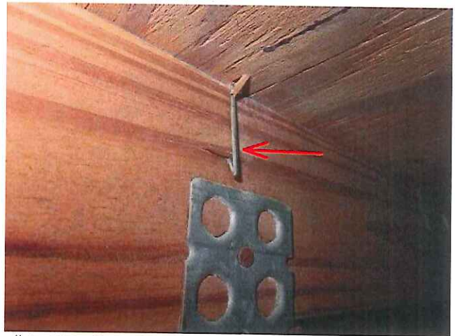
#4 Staples for roof deck attachment
