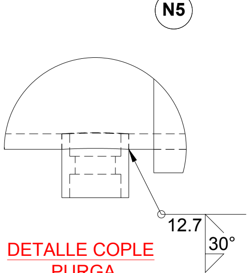
C (1:2)
