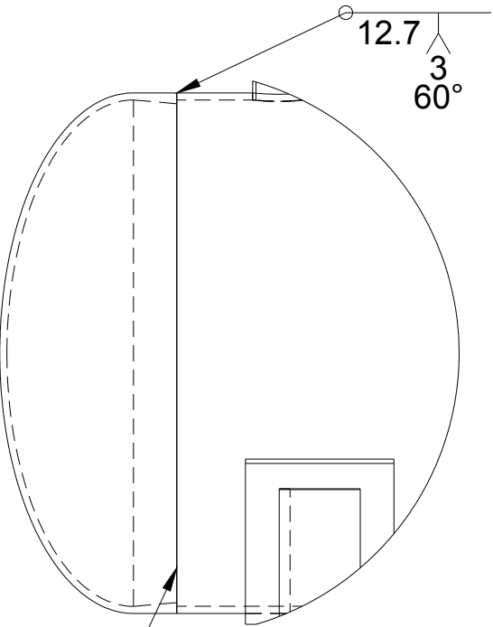
B (1:8)
