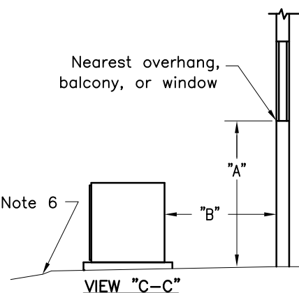
VIEW "C-C"
