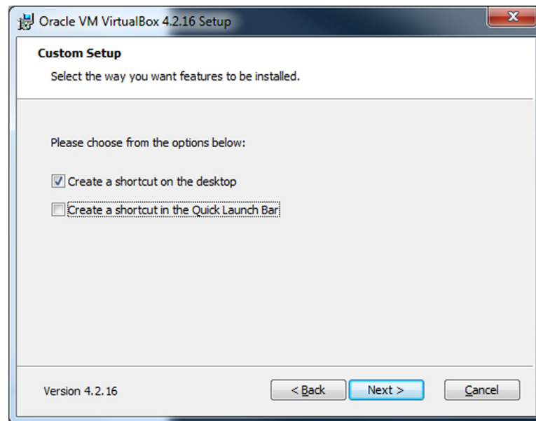
FIGURE 5.3 Installing Virtualbox-3.
