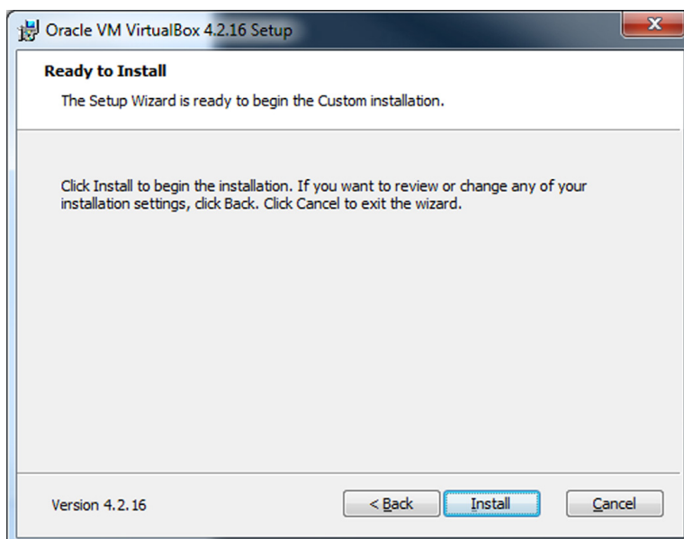
FIGURE 5.5 Installing Virtualbox-5.
