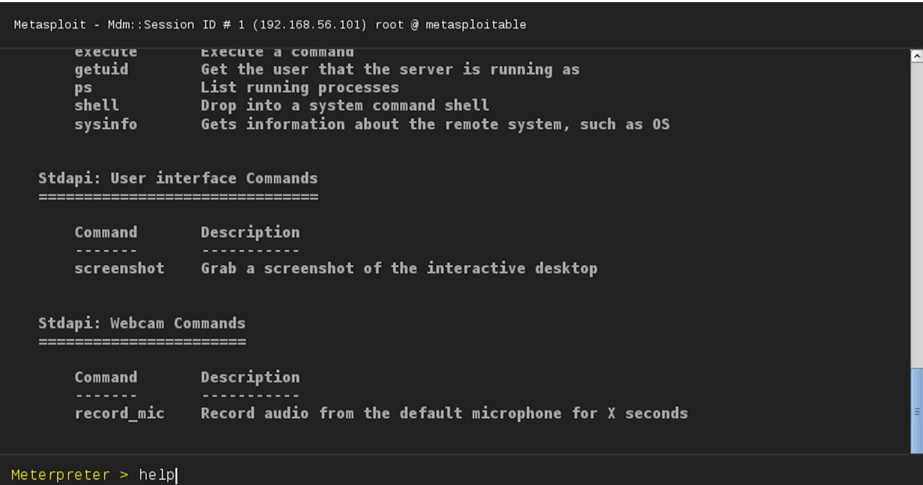
FIGURE 9.15 Command Shell.
