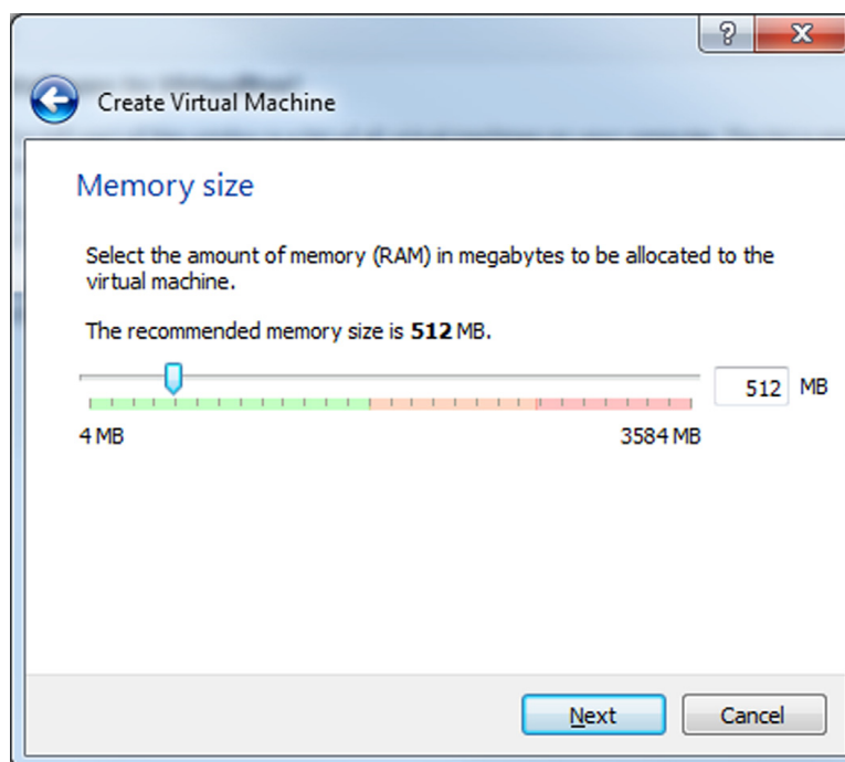
FIGURE 5.22 Configure RAM.
