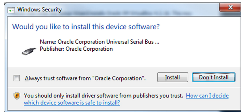
FIGURE 5.6 Installing Virtualbox-6.
