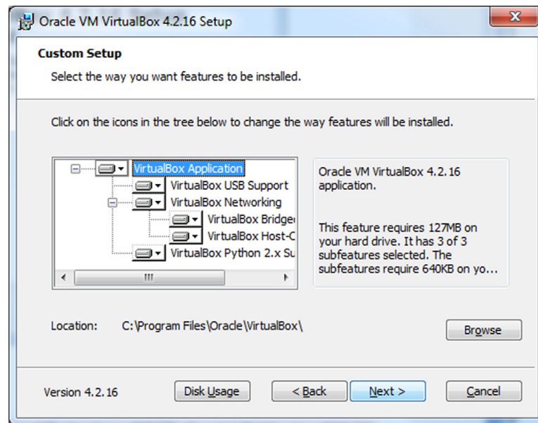
FIGURE 5.2 Installing Virtualbox-2.
