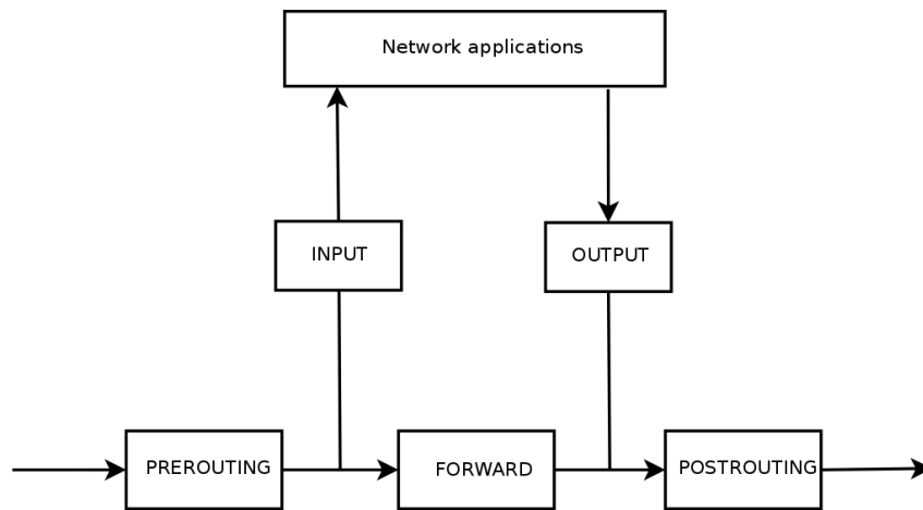
Figure 7.1 How Netfilter Chains are Called
