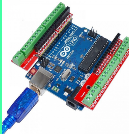
Arduino UNO Screw Shields V2 Terminal Expansion Board
