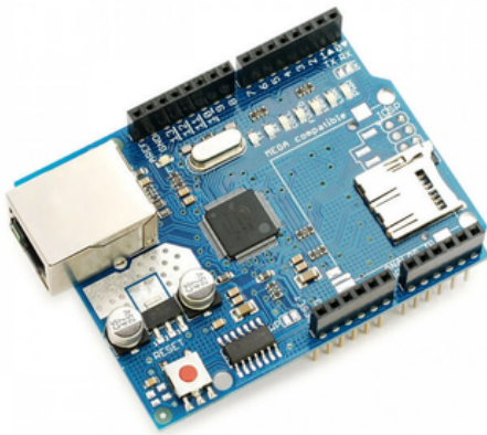
Arduino Ethernet Shield W5100 with Micro SD Card Slot
