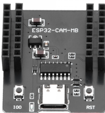
ESP32-CAM-MB Type- C Serial Port Burner Module
