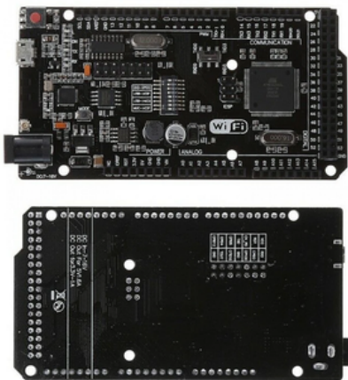
Arduino Mega +WiFi R3 + NodeMCU ESP8266 Board
