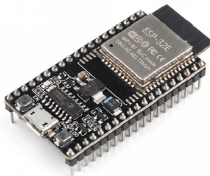
NodeMCU 38-Pin ESP32 Dev. Board with ESP-32E
