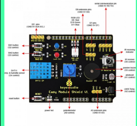
keyestudio Multi-purpose Shield V1
