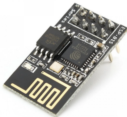
ESP8266 ESP-01 WIFI Transceiver Wireless Module
