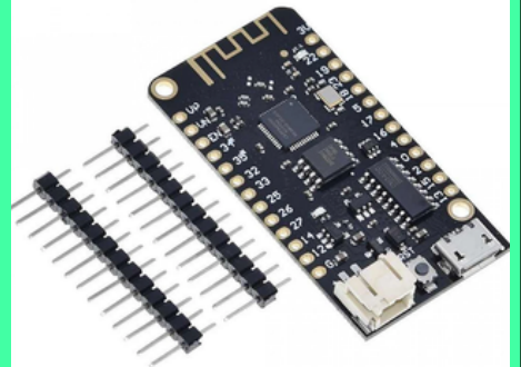
ESP32 V1.0.0 Wifi Bluetooth Development Board
