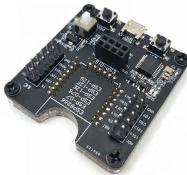
ESP8266 Burn Downloader
