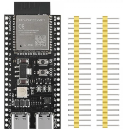
ESP32-S3 N16R8 Development Board - 16MB Flash 8MB
