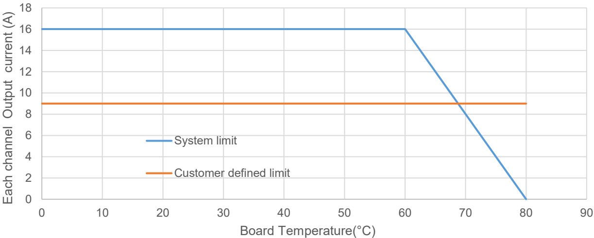
Each channel output current limit Vs Board Temperature
