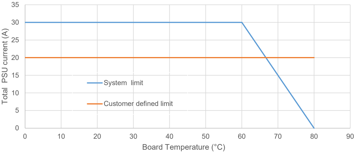
VTC1503 Total PSU current limit Vs Board Temperature
