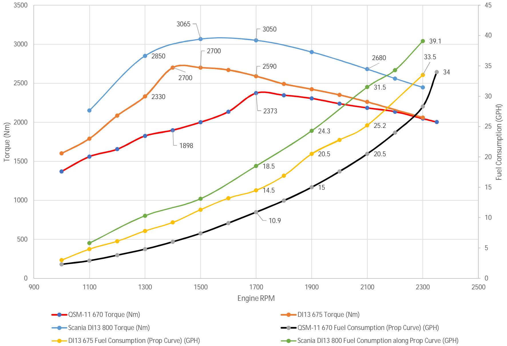
Scania DI13 675 and 800 Hp vs. Cummins QSM-11 670 Mhp Performance Comparison
