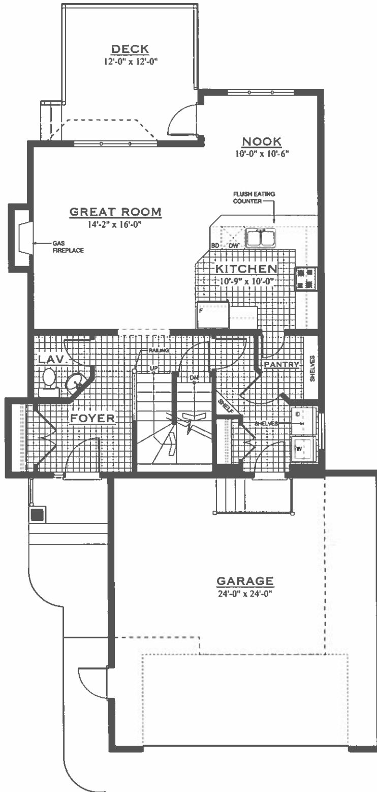
THE WELLINGTON MAIN FLOOR PLAN 830 SQ. FT. 31'-0" WIDE
