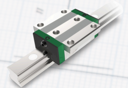
Linear Bearing & Guideway Assembly
