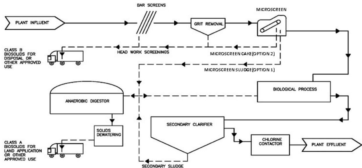
FIGURE 1A – CONVENTIONAL PLANT WITH MICROSCREEN
