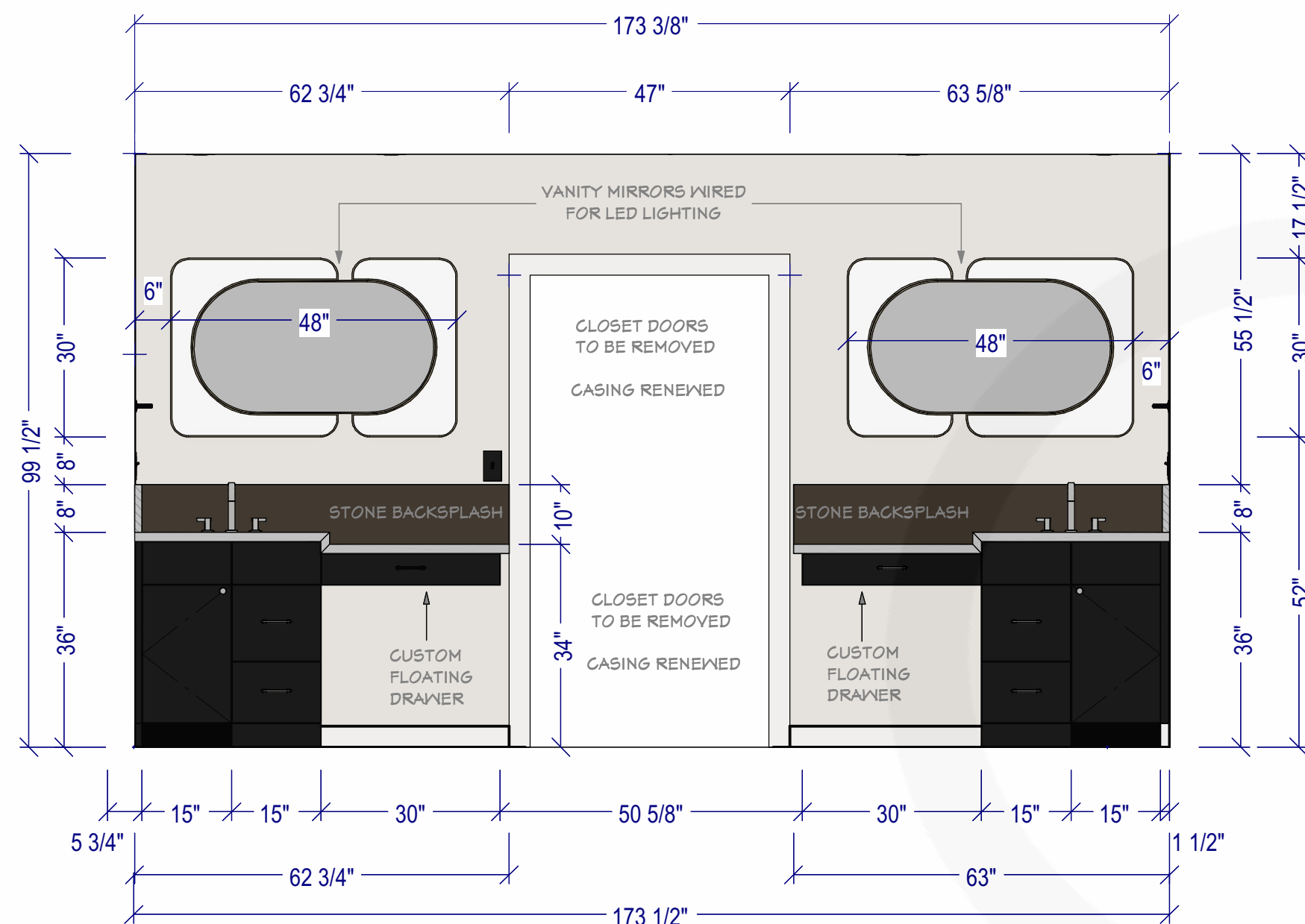
WALL ELEVATION-1 SCALE TO 1/2" = 1' ON ARCH D
