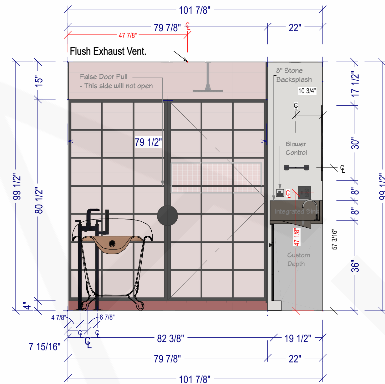
WALL ELEVATION-2 SCALE TO 1/2" = 1' ON ARCH D
