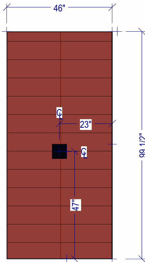
WALL ELEVATION-5 SCALE TO 1/2" = 1' ON ARCH D
