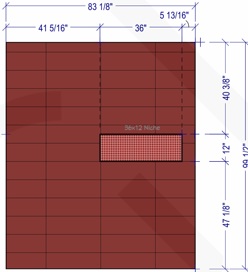
WALL ELEVATION-6 SCALE TO 1/2" = 1' ON ARCH D
