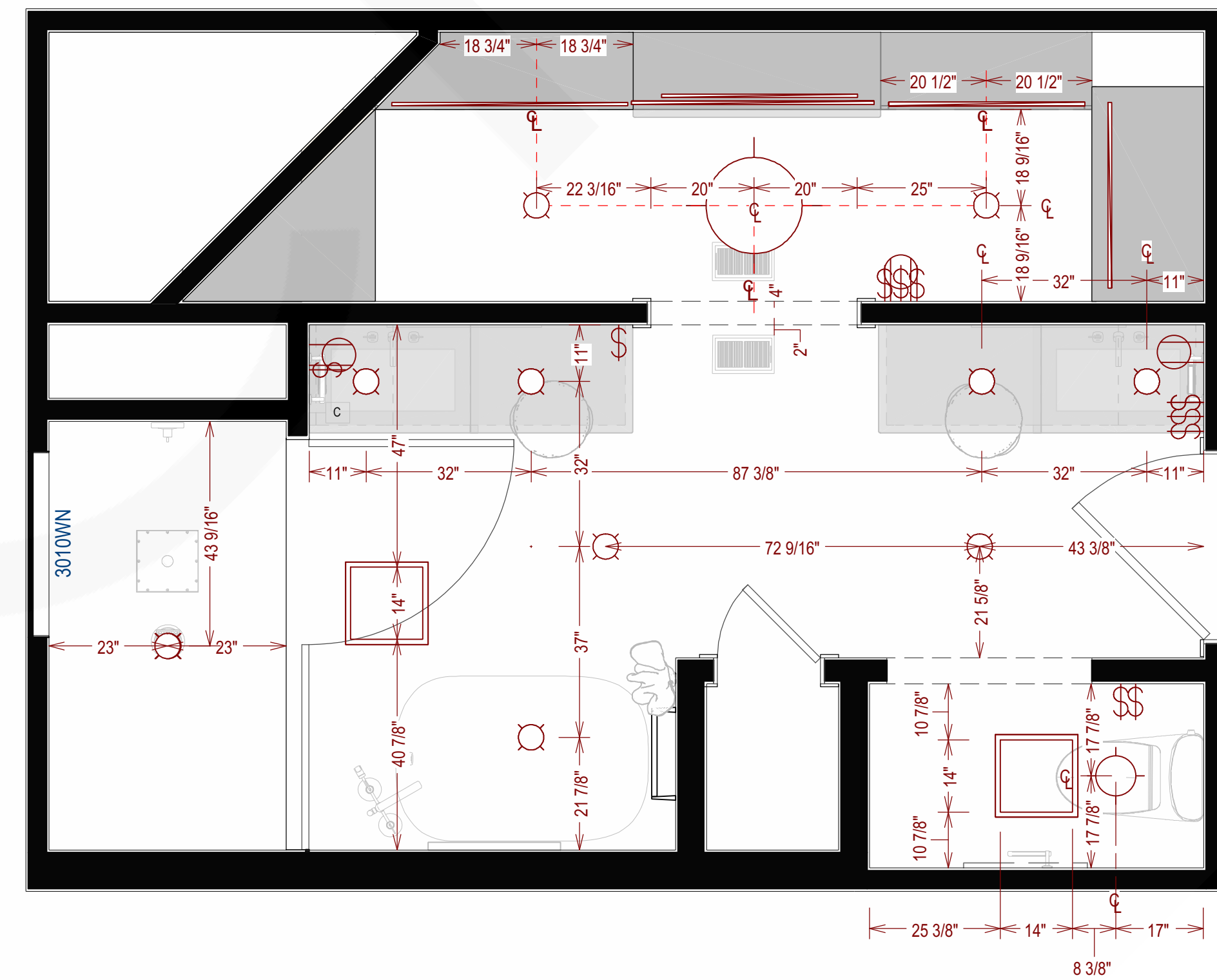
PROPOSED RCP & ELECTRICAL PLAN WITH DIMENSIONS SCALE TO 1/2" = 1' ON ARCH D
