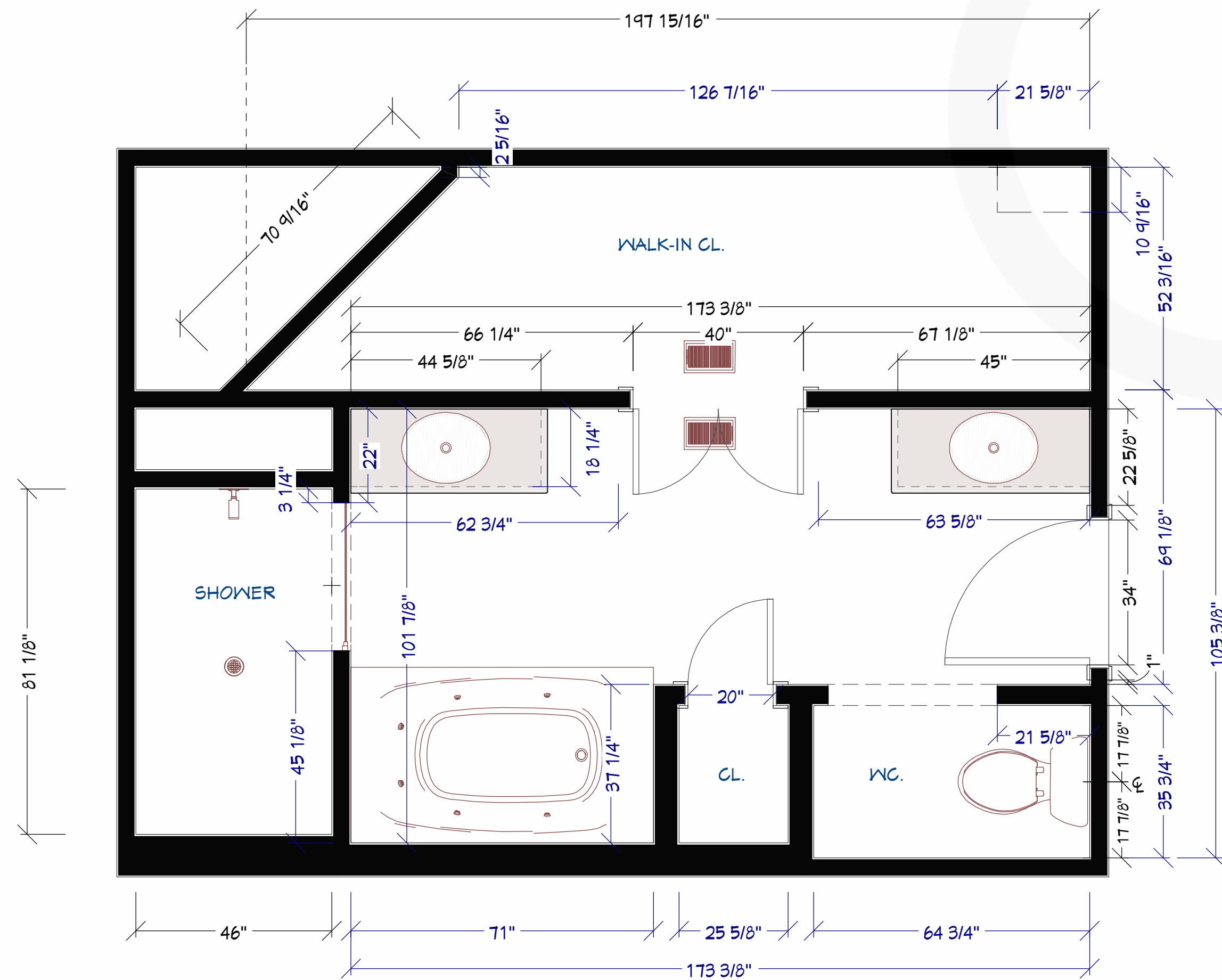
AS-BUILT PLAN SCALE TO 1/2" = 1' ON ARCH D
