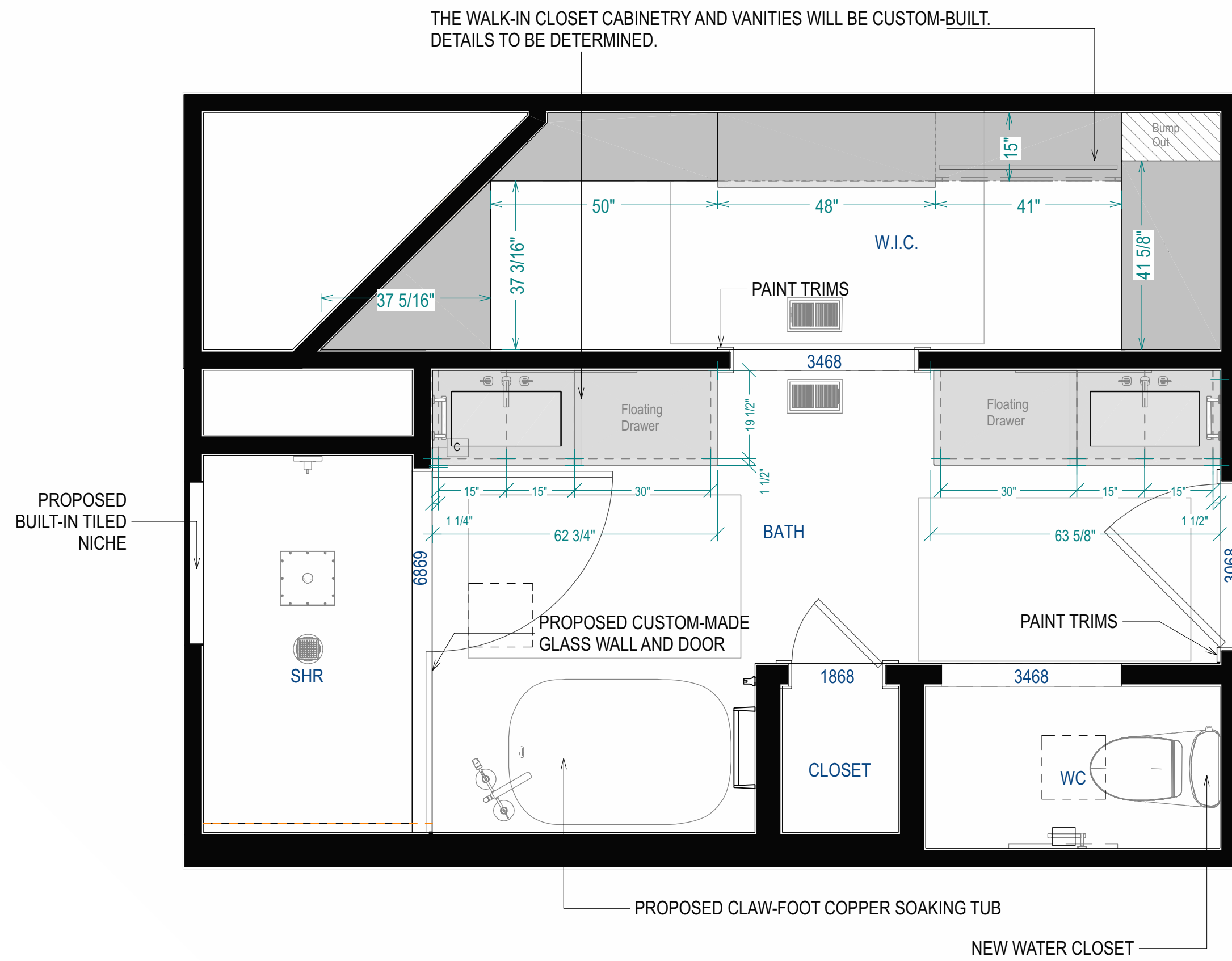
PROPOSED DESIGN w/ CABINETRY & COUNTERTOP DIMENSIONS SCALE TO 1/2" = 1' ON ARCH D
