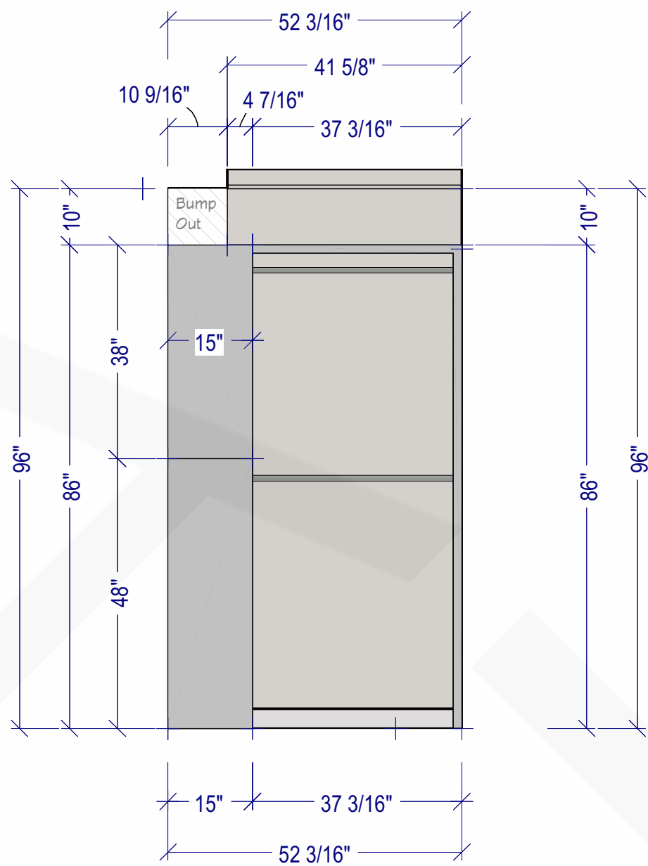
WALL ELEVATION-7 SCALE TO 1/2" = 1' ON ARCH D
