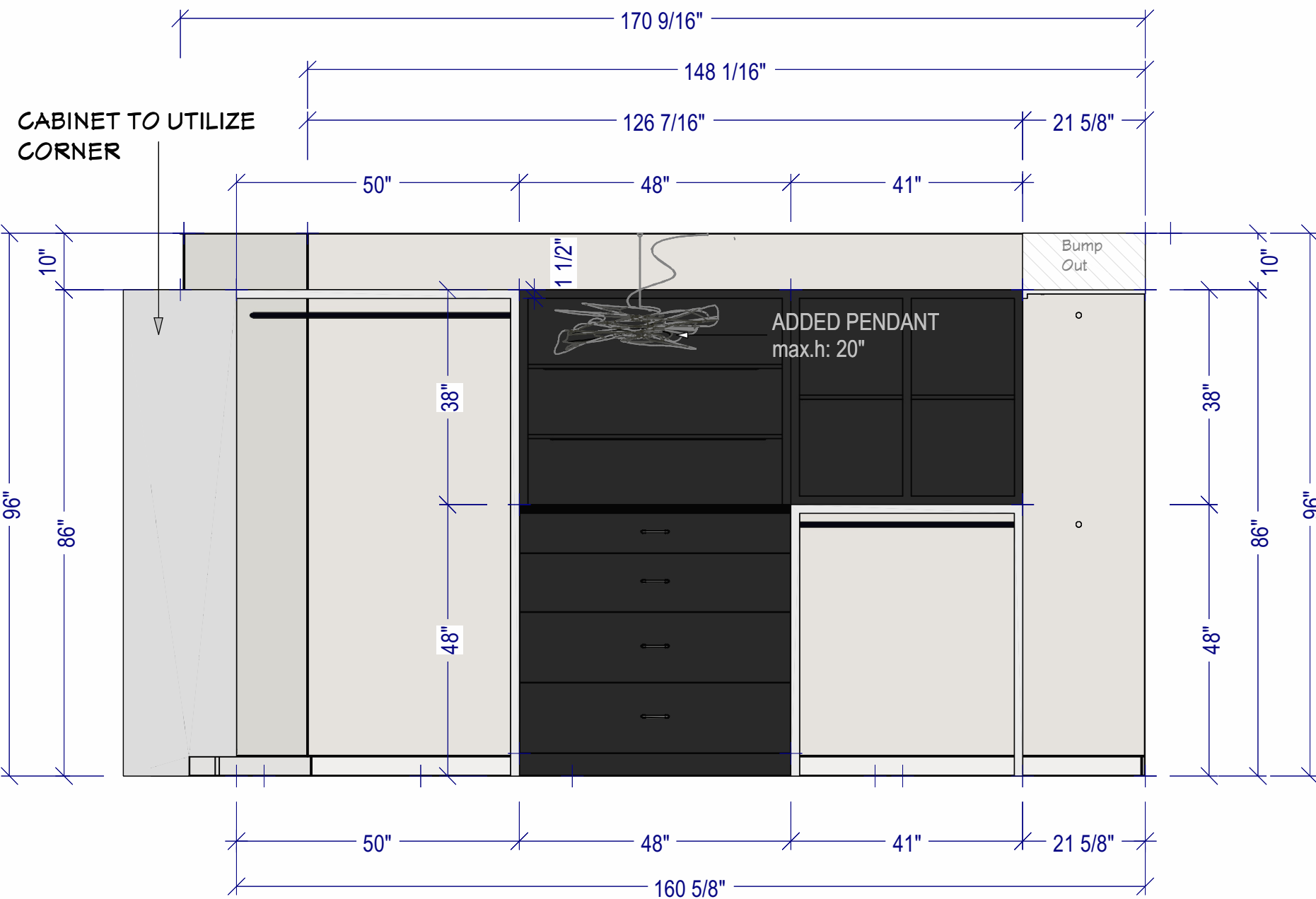
WALL ELEVATION-8 SCALE TO 1/2" = 1' ON ARCH D
