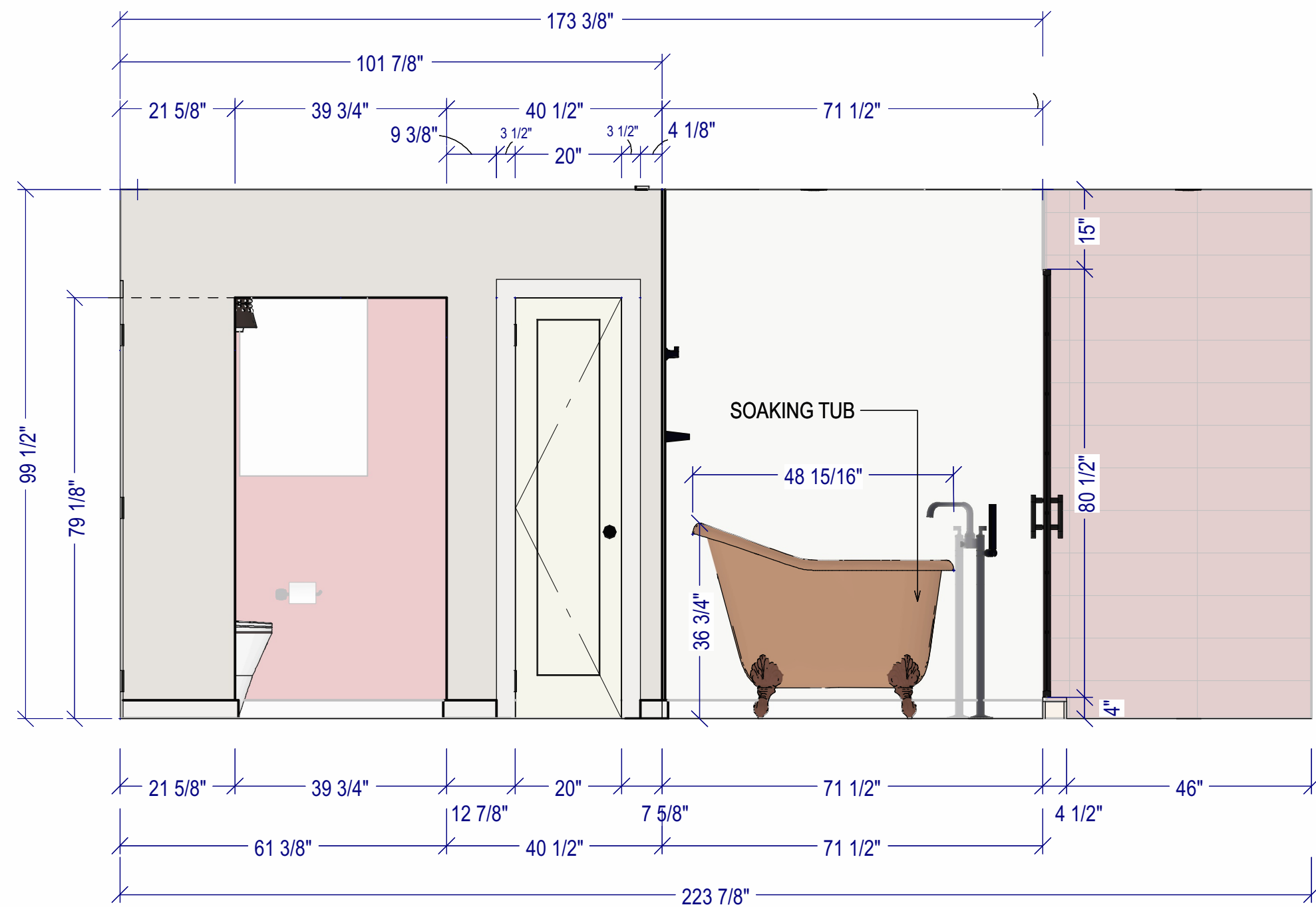
WALL ELEVATION-3 SCALE TO 1/2" = 1' ON ARCH D
