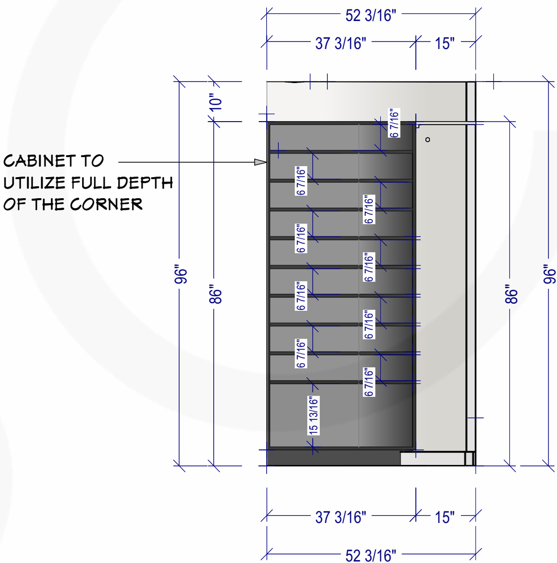
WALL ELEVATION-9 SCALE TO 1/2" = 1' ON ARCH D
