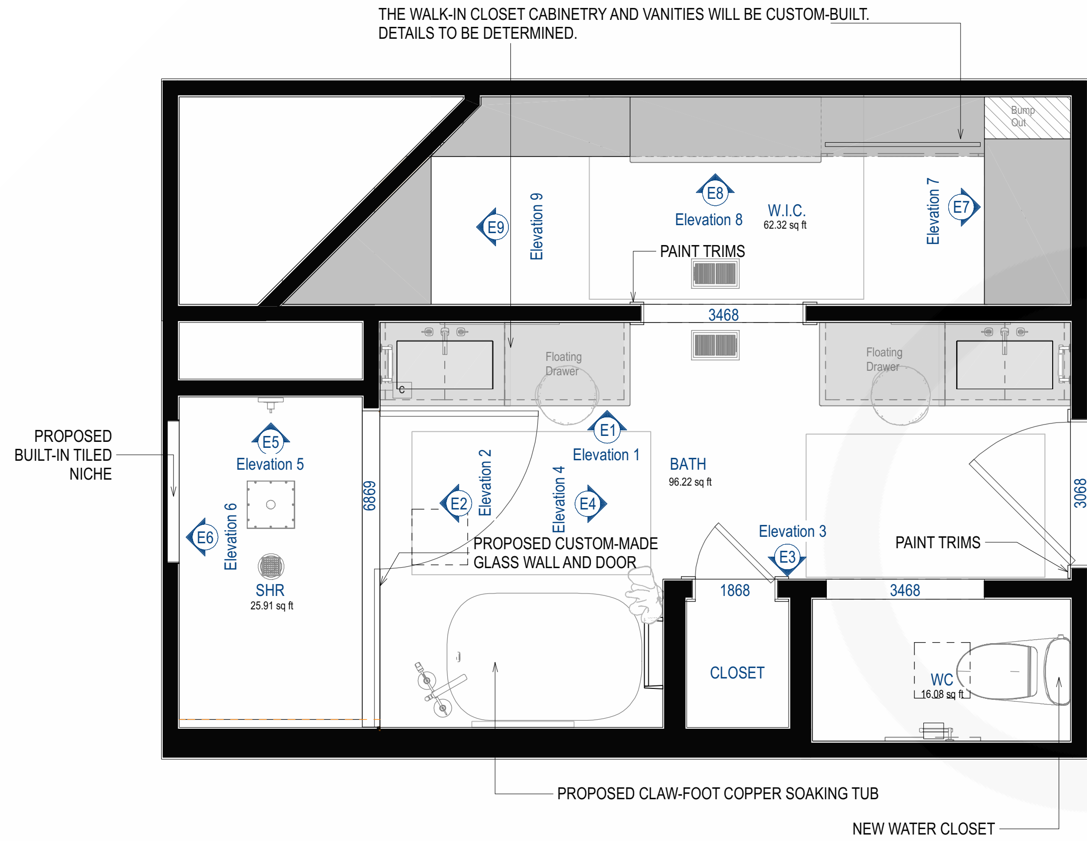
PROPOSED FLOOR PLAN SCALE TO 1/2" = 1' ON ARCH D
