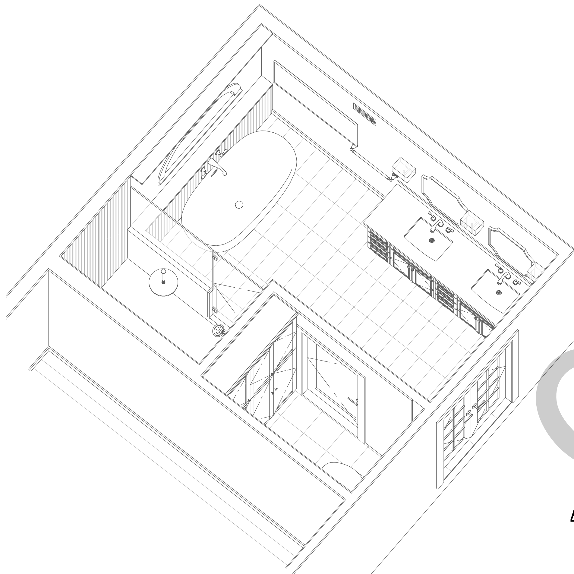
AXONOMETRIC FLOOR OVERVIEW 1/2":1'
