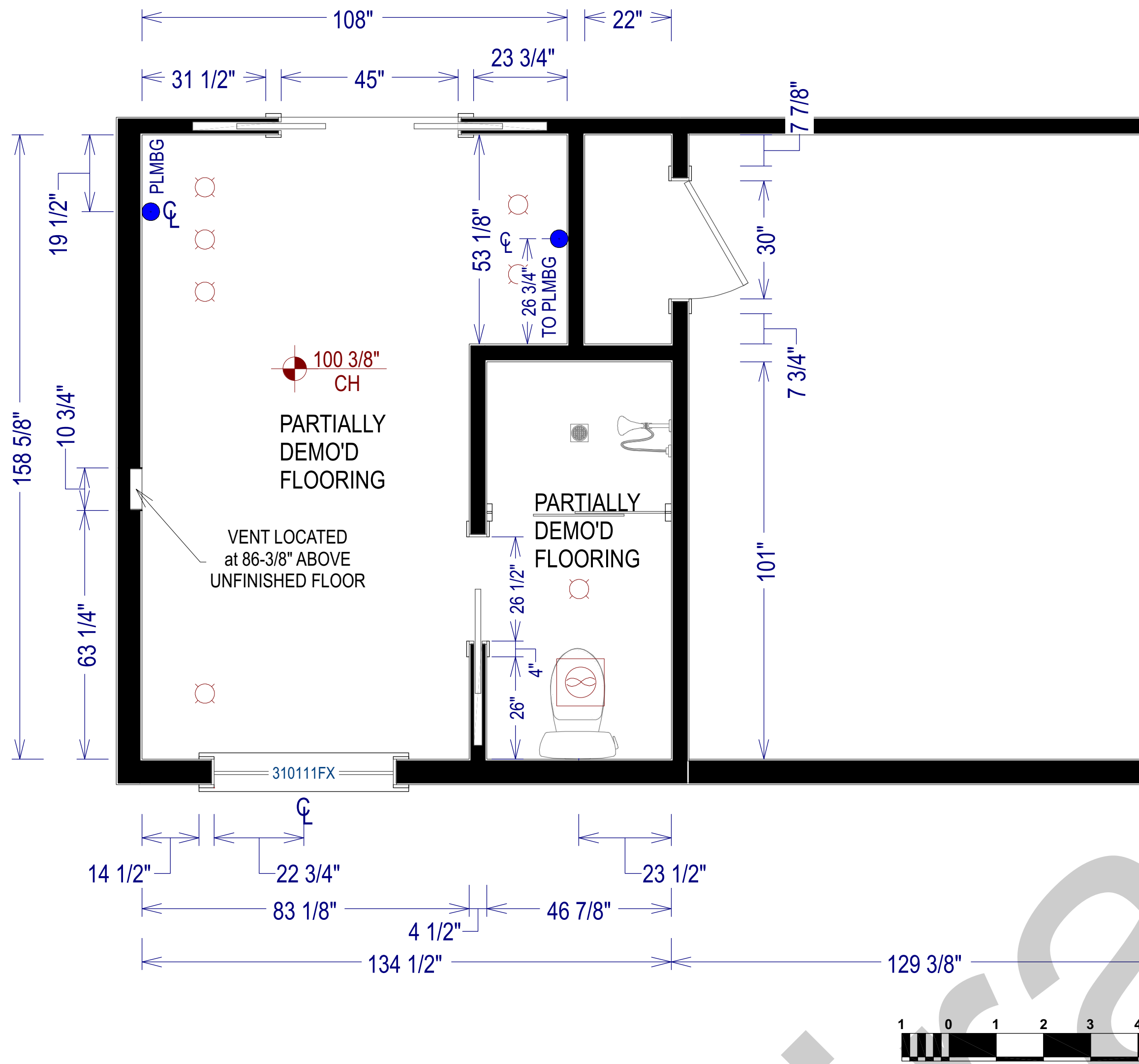
AS-BUILT FLOOR PLAN SCALE TO 1/2" = 1' ON ARCH D
