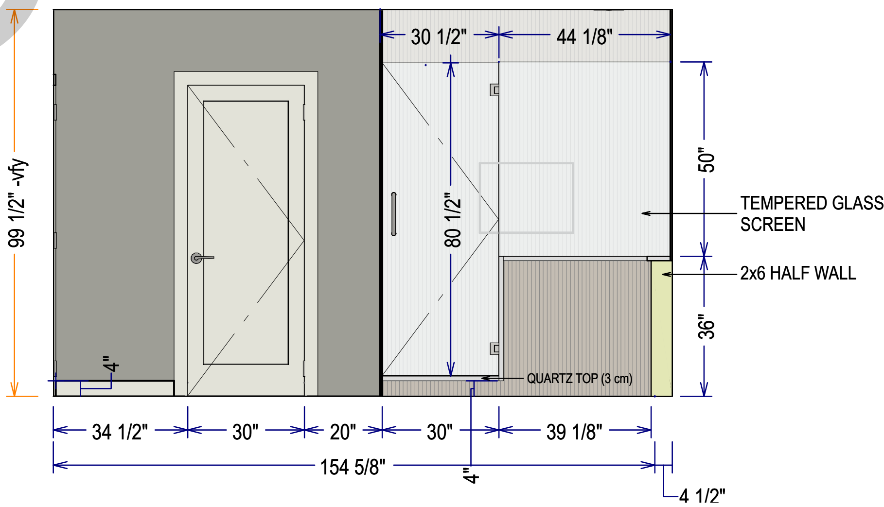
ELEVATION-4 SCALE TO 1/2" = 1' ON ARCH D
