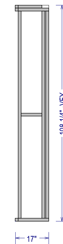
WALL DETAIL-4 SCALE TO 1/2" = 1' ON ARCH D
