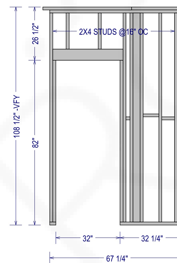
WALL DETAIL-3 SCALE TO 1/2" = 1' ON ARCH D
