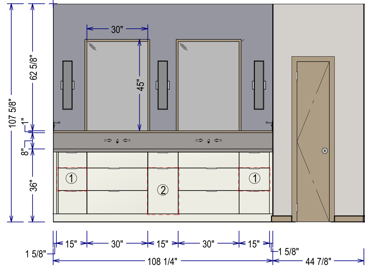
PRIMARY BATH WALL ELEVATION-1 SCALE TO 1/2" = 1' ON ARCH D
