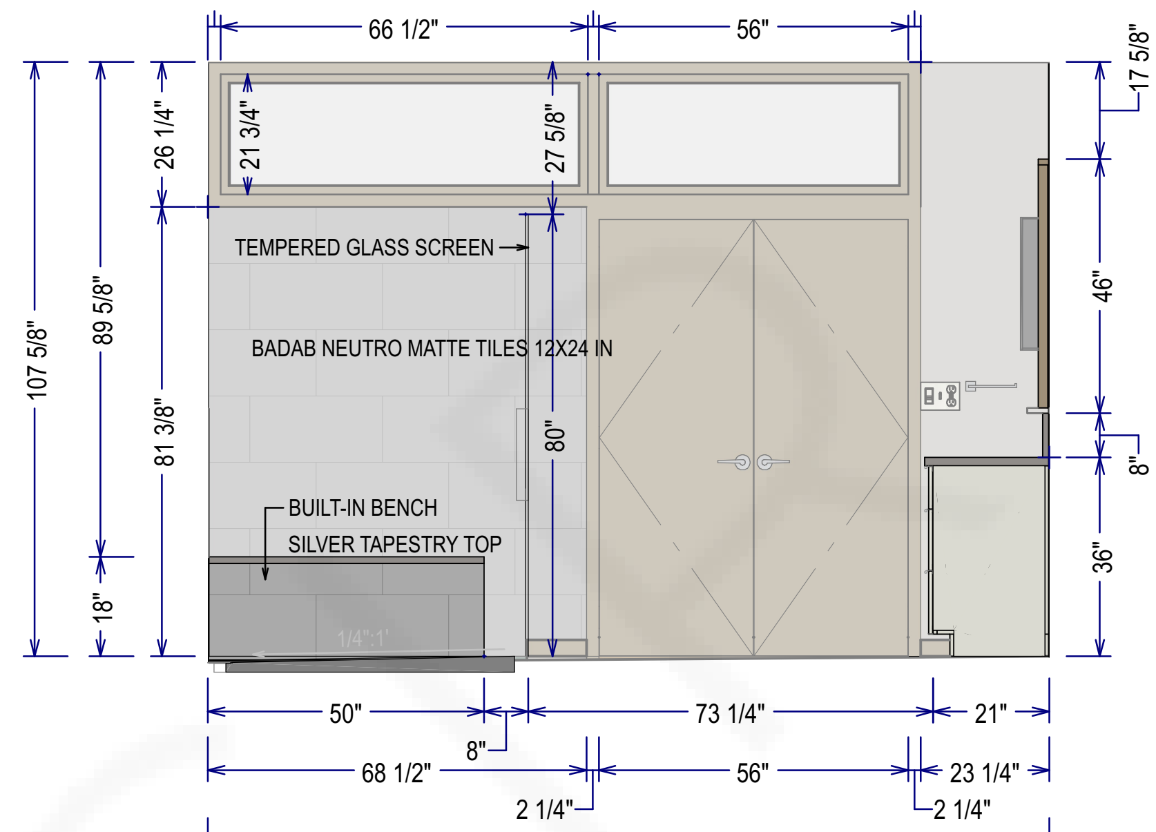
PRIMARY BATH WALL ELEVATION-2 SCALE TO 1/2" = 1' ON ARCH D
