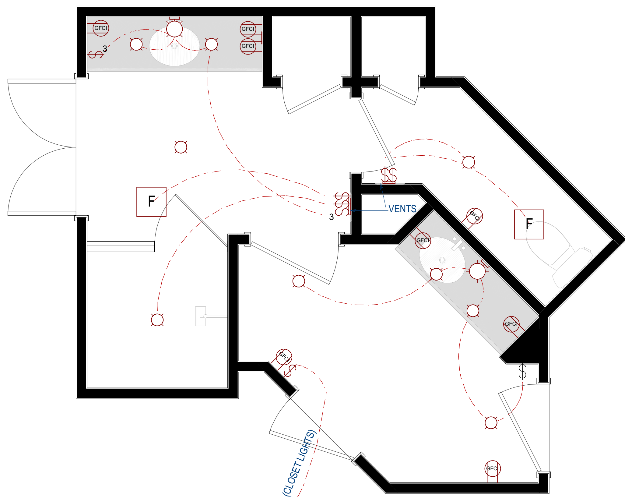
AS-BUILT PLAN SCALE TO 1/2" = 1' ON ARCH D
