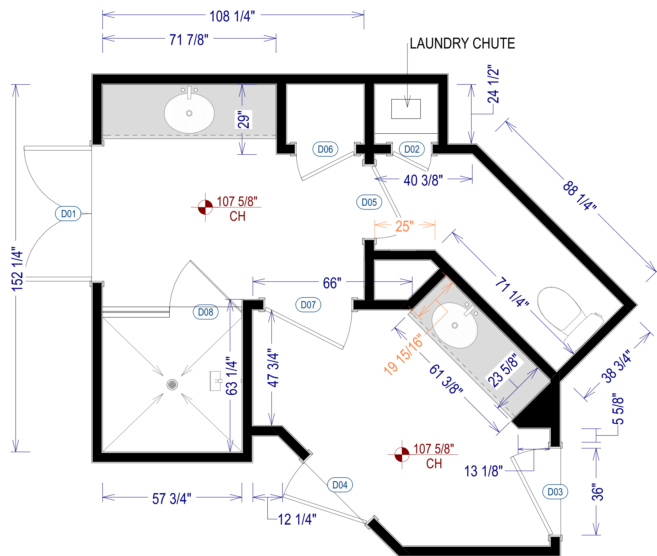
DIMENSIONED AS-BUILT PLAN SCALE TO 1/2" = 1' ON ARCH D
