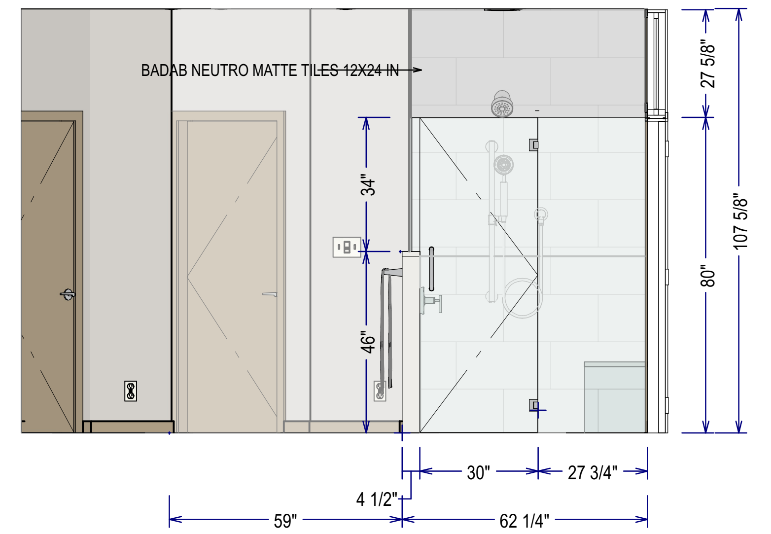
PRIMARY BATH WALL ELEVATION-3 SCALE TO 1/2" = 1' ON ARCH D
