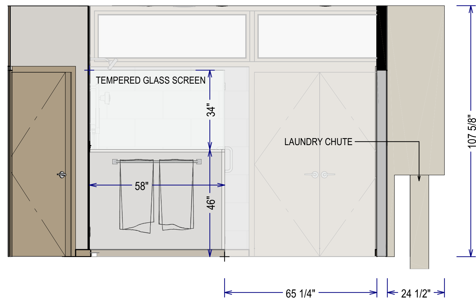
PRIMARY BATH WALL ELEVATION-4 SCALE TO 1/2" = 1' ON ARCH D
