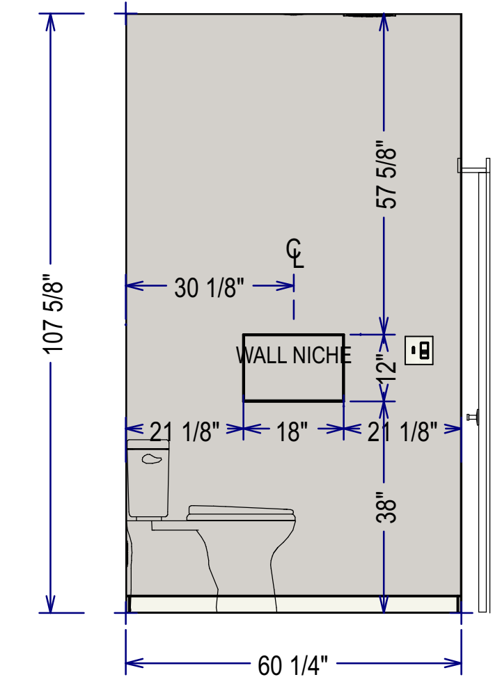
PRIMARY BATH WALL ELEVATION-6 SCALE TO 1/2" = 1' ON ARCH D
