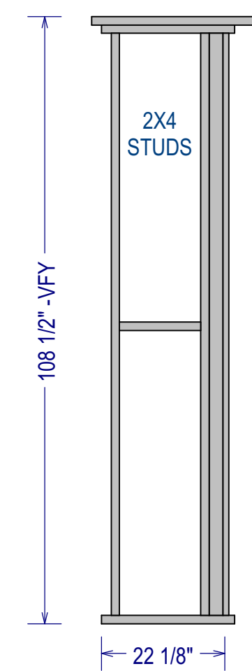
WALL DETAIL-2 SCALE TO 1/2" = 1' ON ARCH D
