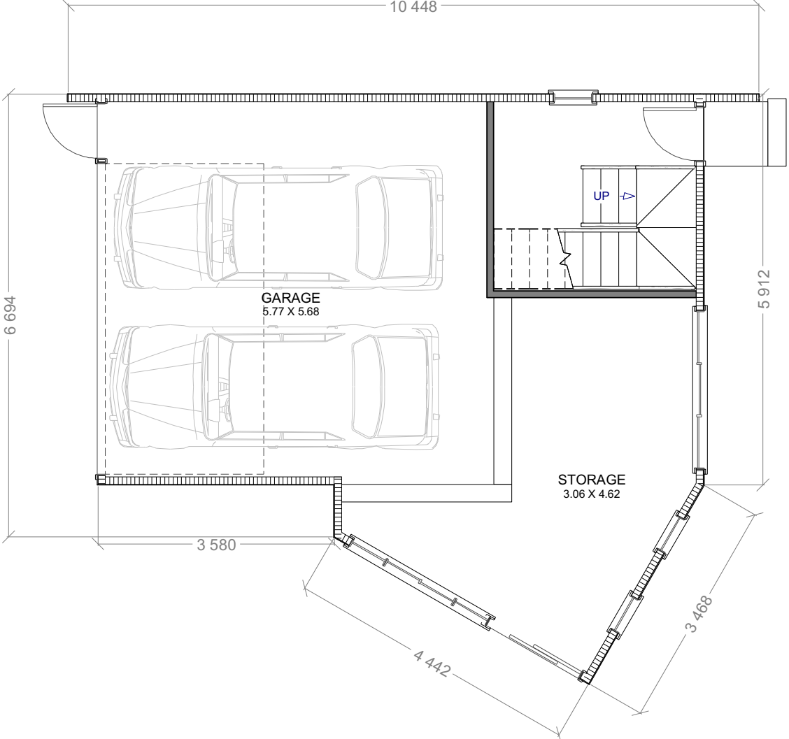
LOWER FLOOR PLAN
