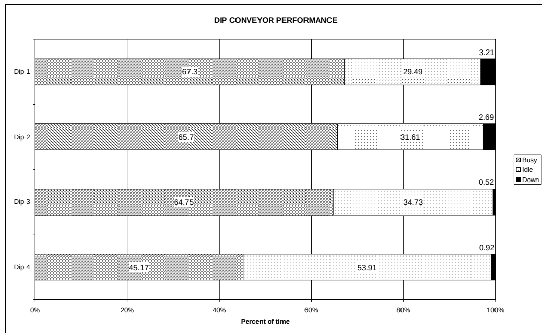
Fig 11: Example of decline conveyor utilisation
