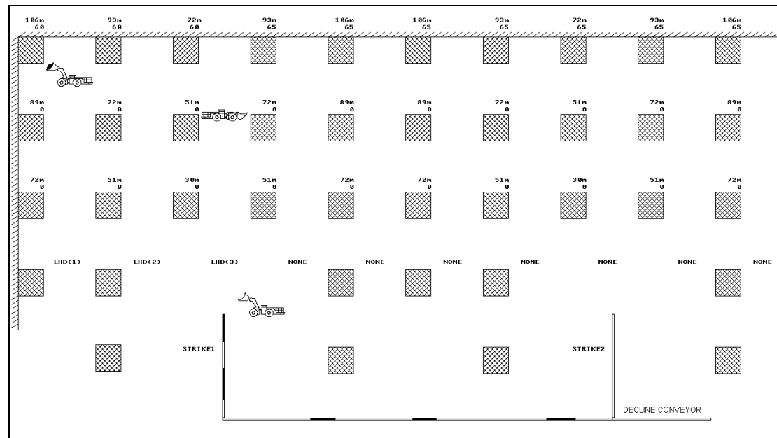
Fig 5: Discrete flow of material on conveyors loaded with LHD direct tipping
