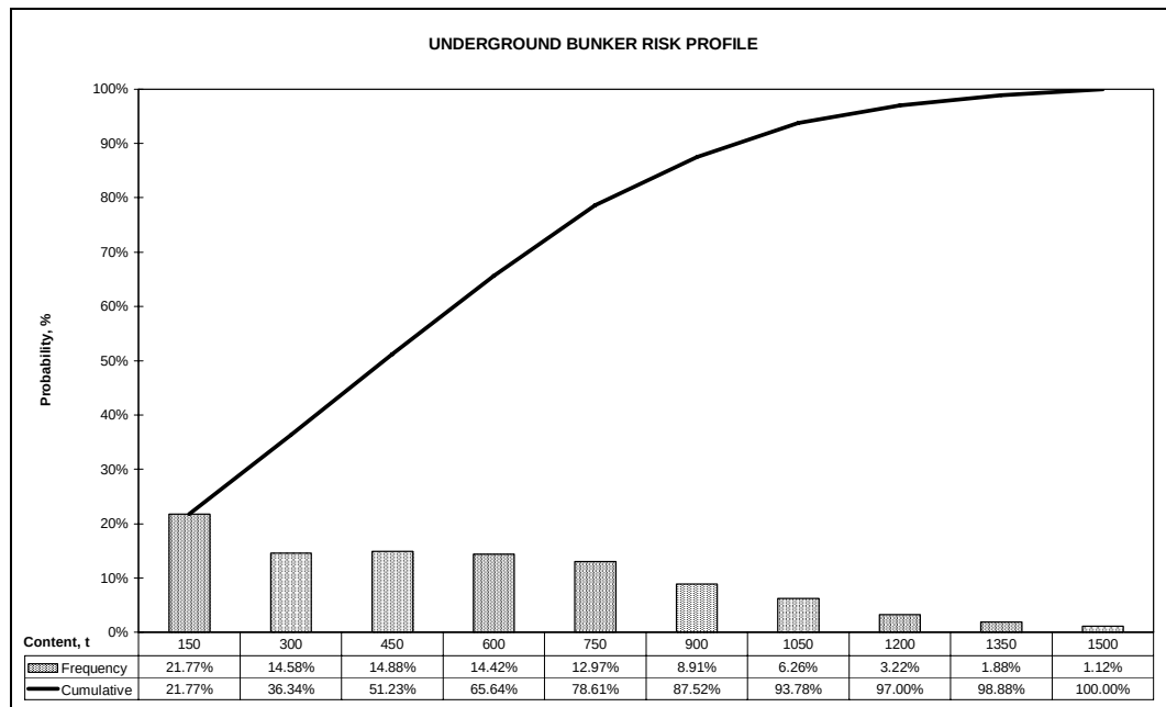
Fig 14: Underground bunker risk profile
