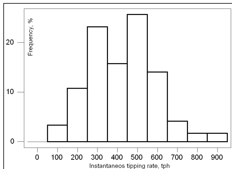
Fig 3: Example of an instantaneous loading rate of a strike conveyor
