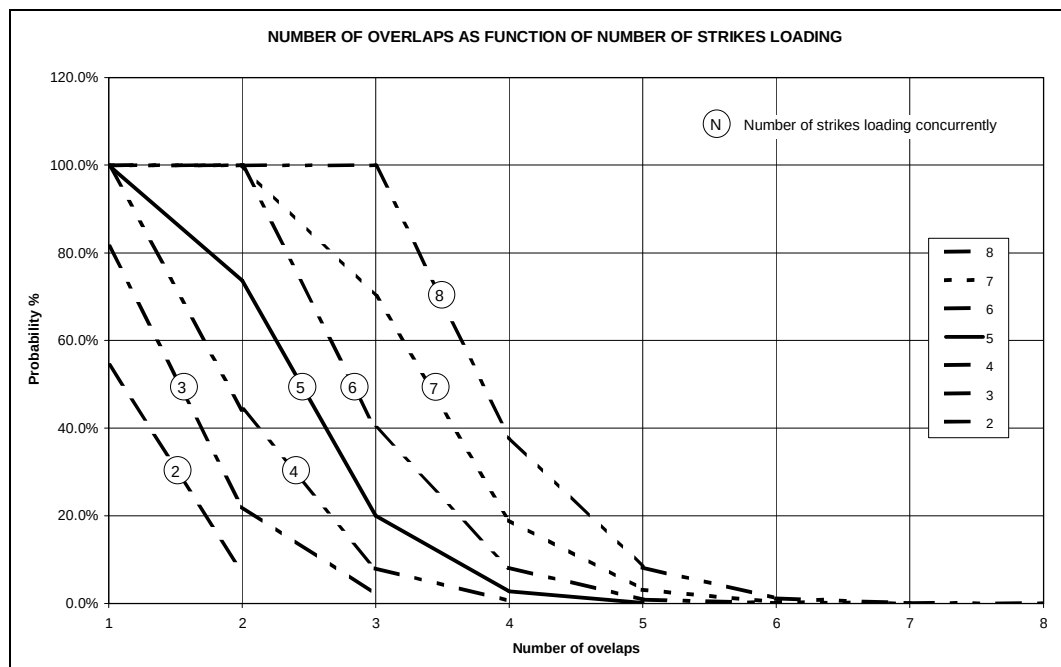
Fig 10: Multi-layering effect on decline belt
