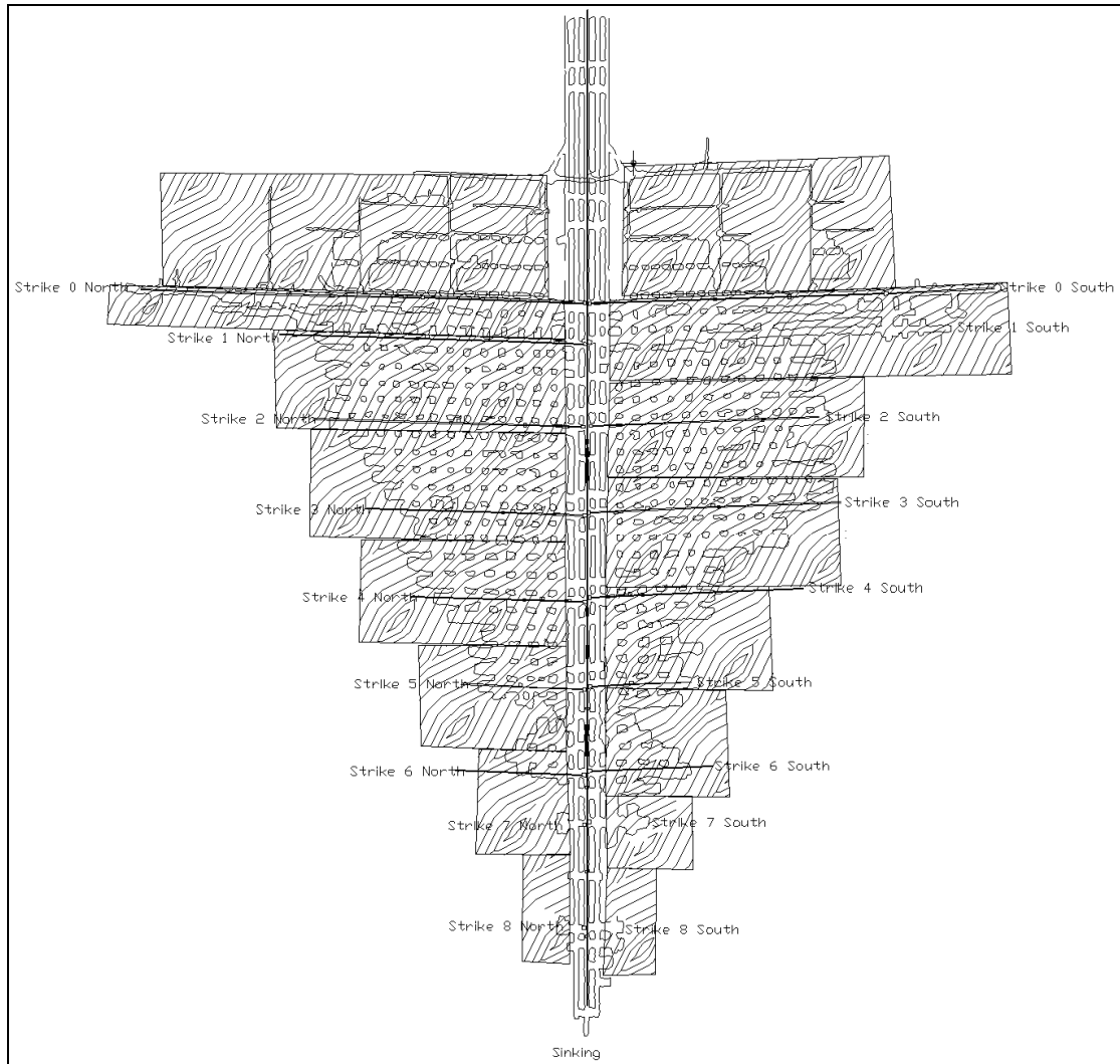
Fig 1: Plan over a conveyor system in an underground on-reef room-and-pillar mine
