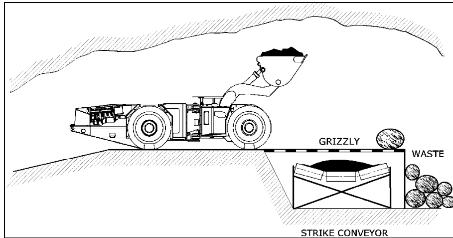
Fig 2: LHD tipping onto the grizzly
