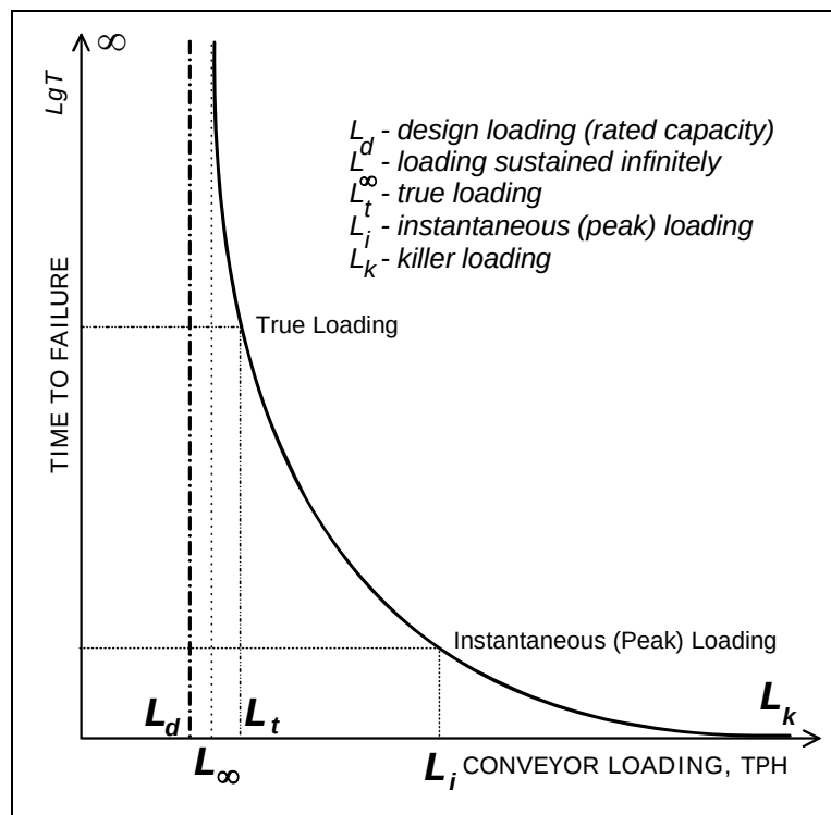
Fig 9: Illustrative correlation between conveyor loading and time it can be sustained (time to failure)
