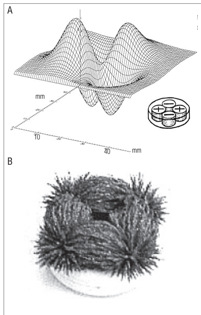
Figure 2. Representation of a quadripolar magnetic array. A: Field map of a quadripolar magnetic array. The magnet arrangement within the device is shown in the lower right corner (Extract from McLean et al. 7 ). B: Pattern produced in iron filings by a quadripolar magnetic array.
