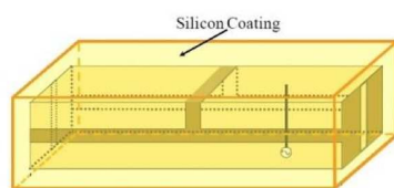
Figure 3.1: Miniaturized cavity slot antennas (reproduced from [19])
