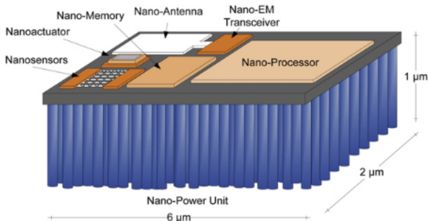
Figure 2.1: An integrated nanosensordevice [28].
