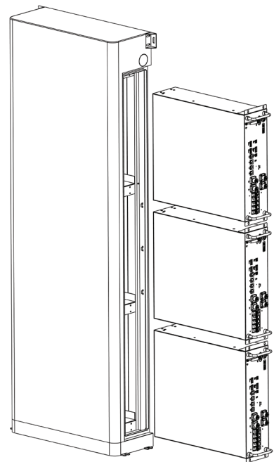
Exploded View
