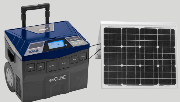
enCUBE battery inverter with 60-watt solar panel
