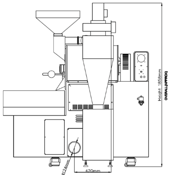
2023/24 BC-25 Drawings
