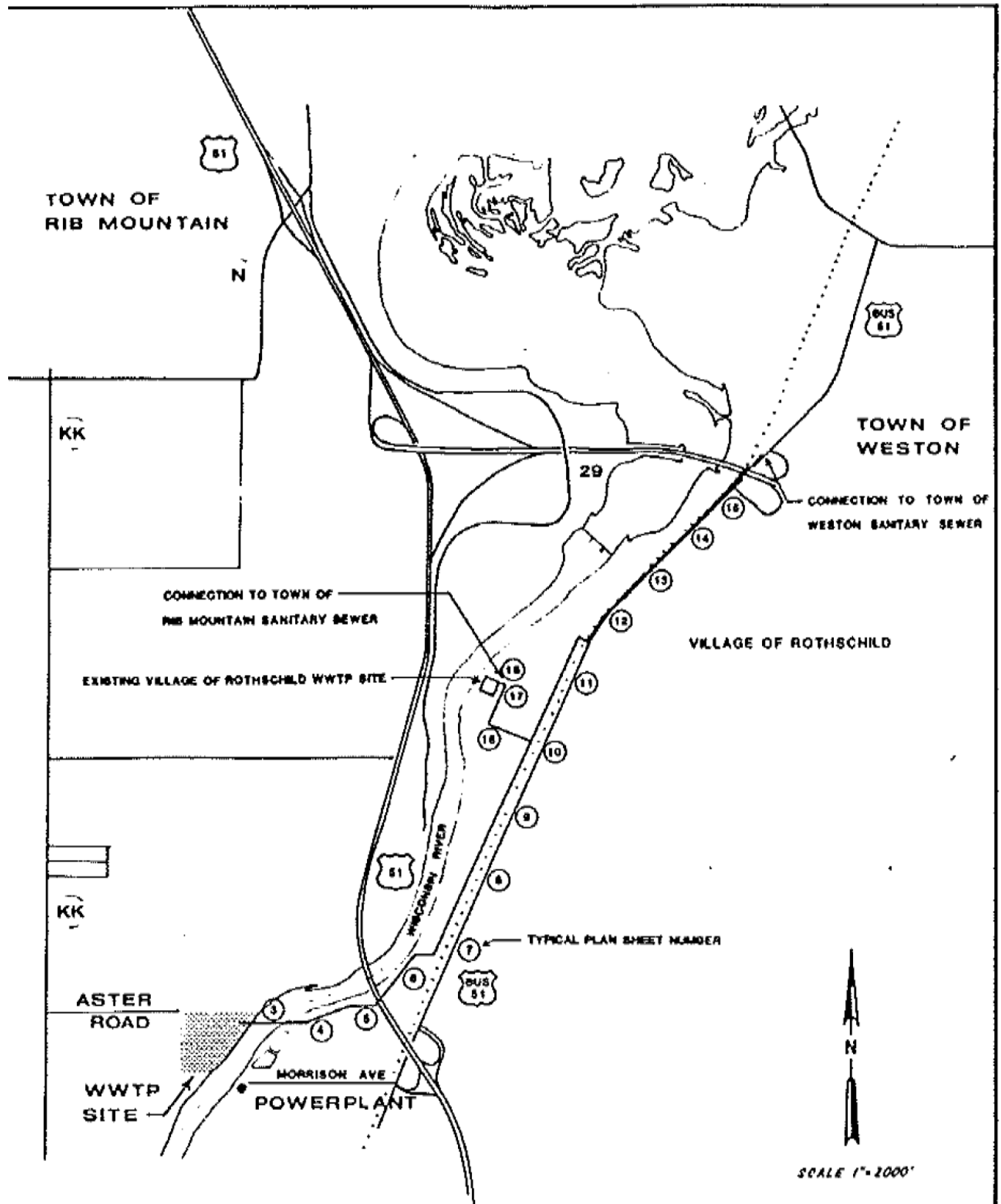
LOCATION PLAN
