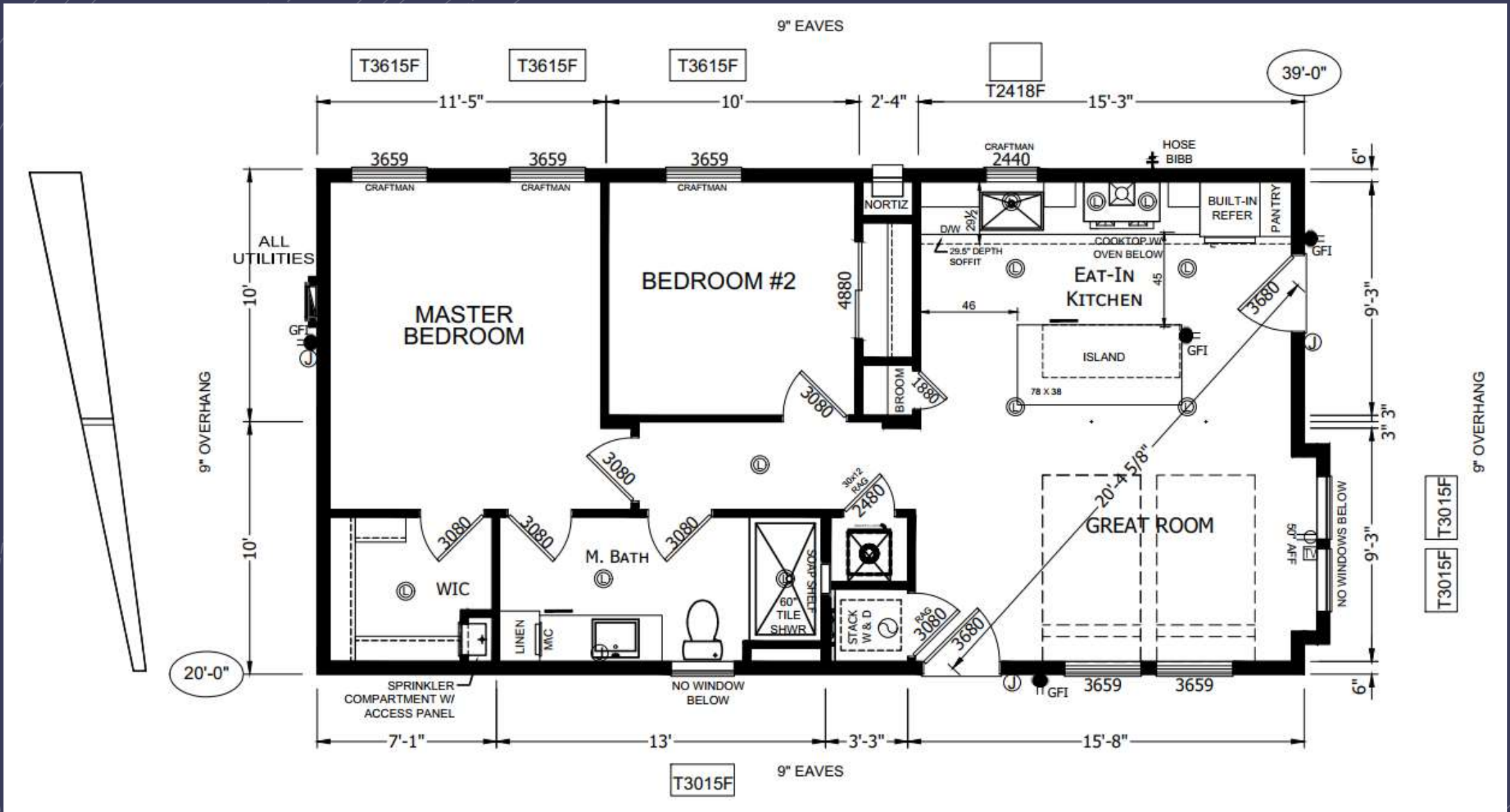
Floor Plan of Genesis ADU 790 Factory Display
